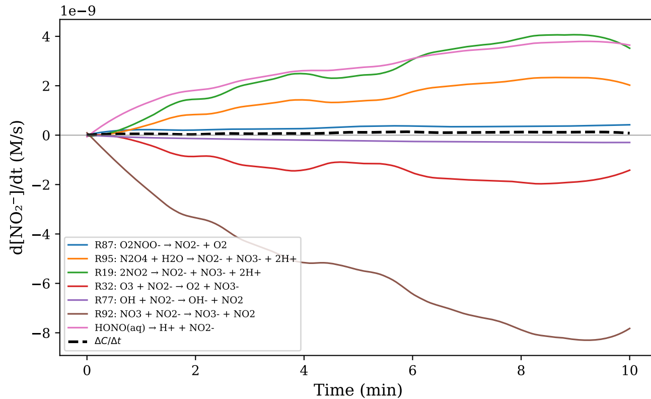
(c) \text{NO}_2^-
