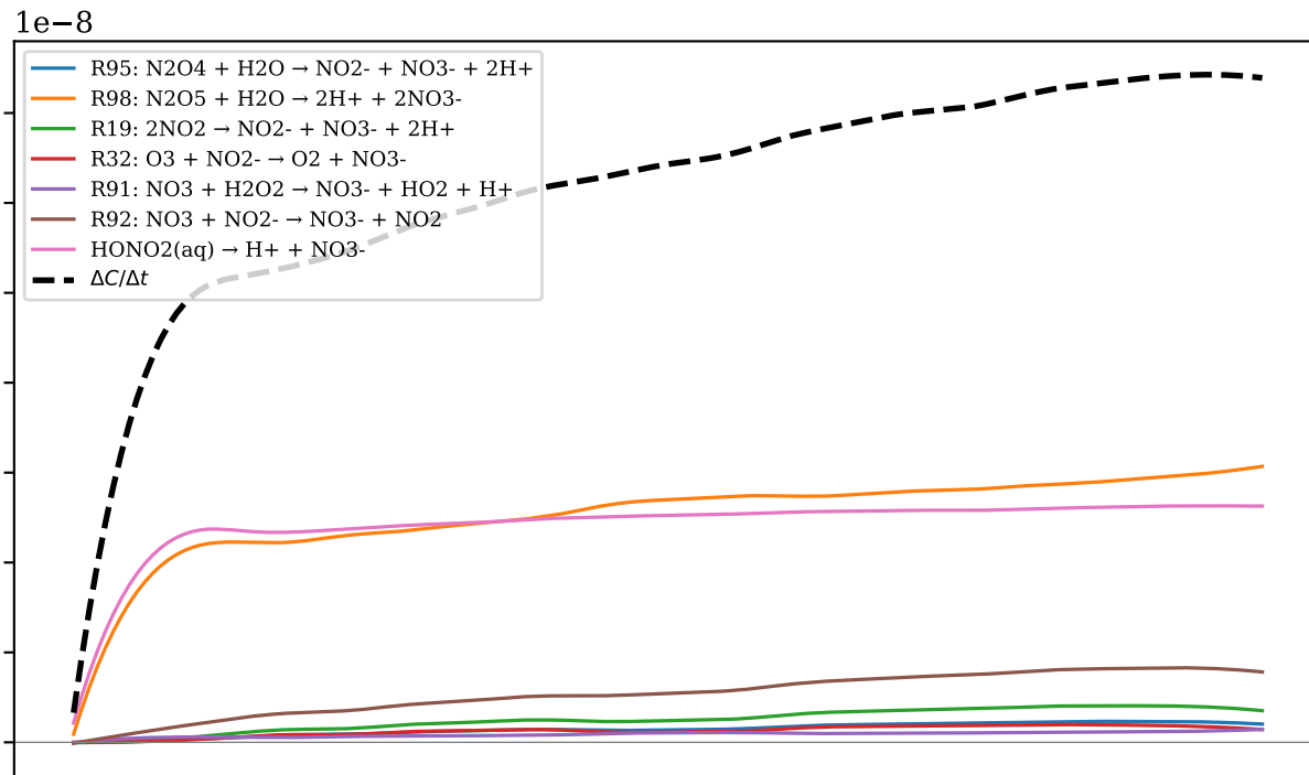
(a) \text{NO}_3^-
